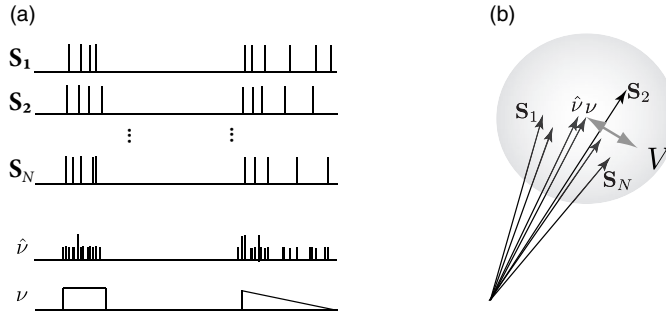
Fig. 10.8 The spike density vector. (a) A set of N spike trains ( \mathbf{S}_1, \mathbf{S}_2, \dots, \mathbf{S}_N ) is combined to yield an estimate of the spike density \hat{\nu} . At the limit N \rightarrow \infty the spike density converges to the instantaneous firing rate \nu . (b) Schematic representation of the quantities in (a). The variability V measures the scatter of the individual spike trains around their mean \hat{\nu}_X .
