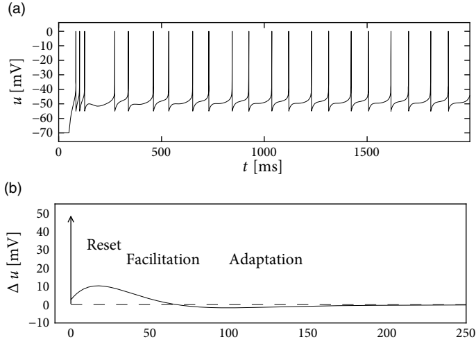
Fig. 6.10 Another type of bursting in a model with two spike-triggered currents. (a) Voltage trace of the neuron model Eqs. (6.3)–(6.4) with u_{\text{reset}} = -55 mV, v_{\text{th}} = -50 mV, b_1 = -12 pA, b_2 = 60 pA, \tau_1 = 20 ms, \tau_2 = 61 ms, a_1 = -3 nS and a_2 = 0 . Parameters were chosen to correspond to a neuron coupled with a dendritic compartment and I_M . (b) Voltage deflection brought by an isolated spike. Each spike brings first refractoriness, then a facilitation and finally adaptation on a longer time scale.
