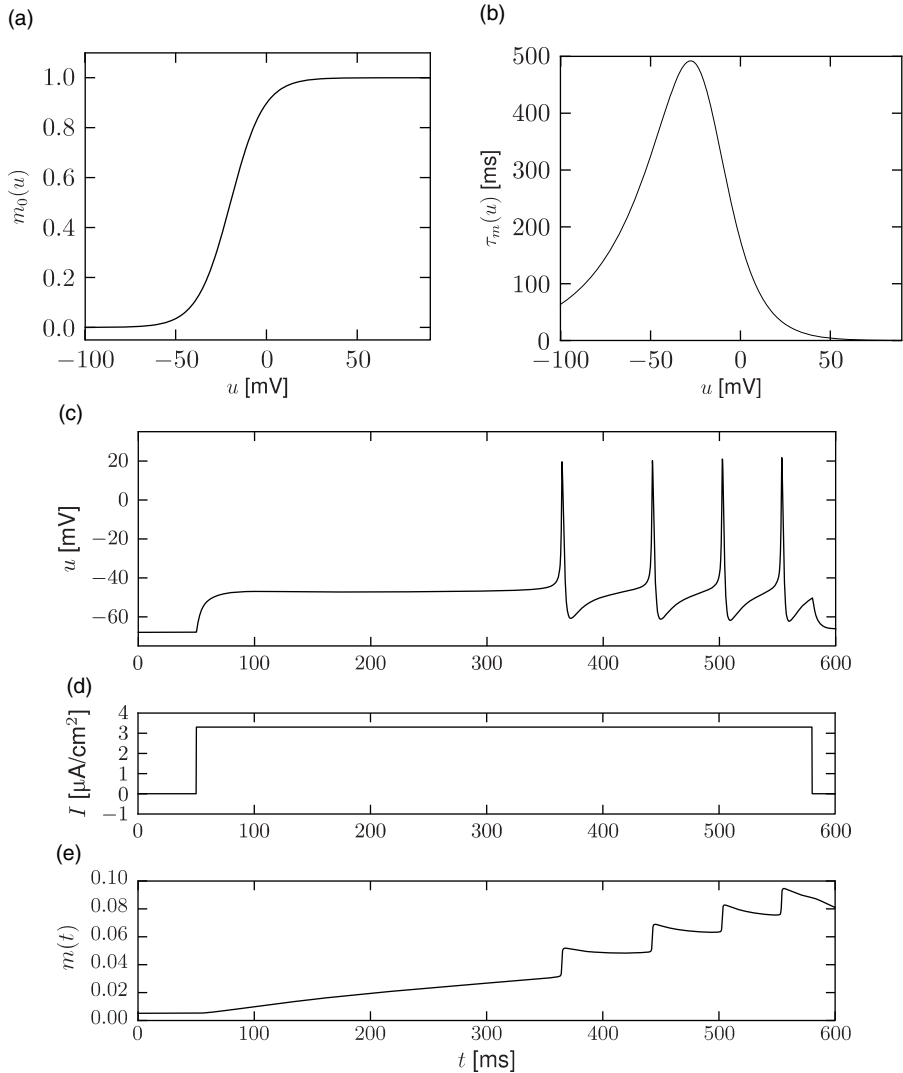
Fig. 2.18 Subthreshold facilitation with I_{\text{NaS}} . (a) Stationary values and (b) time constants of the activation variable m for the slow sodium current I_{\text{NaS}} similar to measurements done in pyramidal neurons of the hippocampus (Hoehn et al. , 1993). (c) Voltage response. (d) External current. (e) Slow sodium current activation, leading to delayed spike initiation and firing frequency facilitation.
