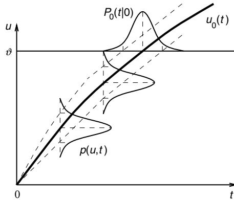
Fig. 8.8 Interval distribution P_0(t|0) for superthreshold stimuli. The membrane potential distribution p(u,t) is shifted across the threshold and generates an interval distribution P_0(t|0) (schematic figure).
