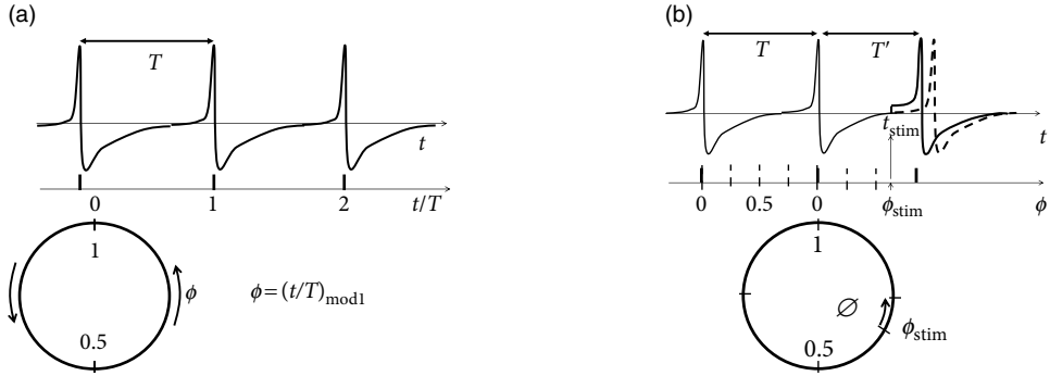
Fig. 20.8 Phase models. (a) For a neuron firing with period T (top), we can introduce a phase variable \phi = (t/T)_{\text{mod}1} (bottom). (b) If a weak input pulse of amplitude \varepsilon is given at a phase \phi_{\text{stim}} , the interspike interval T' is shorter. The phase response curve \tilde{F}(\phi_{\text{stim}}) measures the phase advance \Delta\phi = (T - T')/T as a function of the stimulation phase \phi_{\text{stim}} .
