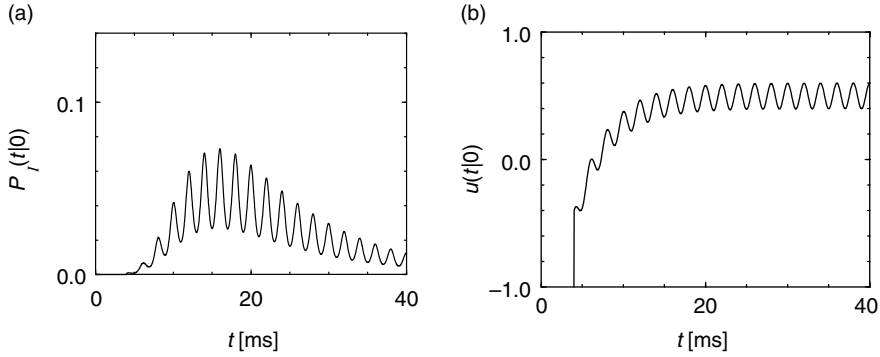
Fig. 9.8 (a) Input-dependent interval distribution P_I(t|0) for an SRM 0 neuron as in Fig. 9.7 stimulated by a periodically modulated input field h(t) = h_0 + h_1 \cos(2\pi ft) with h_0 = 0.5 , h_1 = 0.1 , and frequency f = 500 Hz. (b) The membrane potential u(t|0) = \eta(t) + h(t) during stimulation as in (a).
