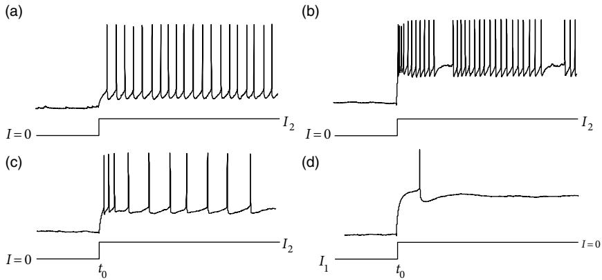
Fig. 1.10 Response to a current step. In (a)–(c), the current is switched on at t = t_0 to a value I_2 > 0 . Fast-spiking neurons (a) have short interspike intervals without adaptation while regularly spiking neurons (c) exhibit adaptation, visible as an increase in the duration of interspike intervals. An example of a stuttering neuron is shown in (b). Many neurons emit an inhibitory rebound spike (d) after an inhibitory current I_1 < 0 is switched off. Data is courtesy of Henry Markram and Maria Toledo-Rodriguez (Markram et al. , 2004; Toledo-Rodriguez et al. , 2004).
