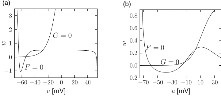
Fig. 4.3 Phase plane u, w of a Hodgkin–Huxley model reduced to two dimensions. (a) The reduction of the Hodgkin–Huxley model leads to a system of two equations, \tau du/dt = F(u, w) + RI and \tau_w dw/dt = G(u, w) . The ensemble of points with F(u, w) = 0 and G(u, w) = 0 is shown as a function of voltage u and recovery variable w , based on Eqs. (4.3), (4.20) and (4.21). (b) As in (a), but for the Morris–Lecar model (see text for details).
