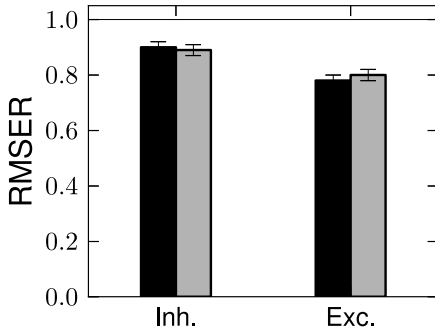
Fig. 11.2 Voltage prediction. Goodness-of-fit of voltage recordings in the main excitatory and inhibitory neuron types of cortical layer 2–3. RMSER (see Chapter 10) for generalized soft-threshold integrate-and-fire models of excitatory and inhibitory neurons (black bars). The gray bars indicate models where the spike-afterpotential is mediated by a spike-triggered change in conductance instead of current. Modified from Mensi et al. (2012).
