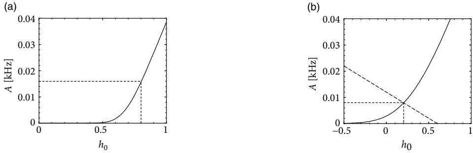
Fig. 12.17 (a) Mean activity of a population of integrate-and-fire neurons with diffusive noise amplitude of \sigma = 0.2 as a function of h_0 = RI_0 . For h_0 = 0.8 the population rate is \nu \approx 16 Hz (dotted line). (b) Mean activity of a population of integrate-and-fire neurons with diffusive noise of \sigma = 0.54 as a function of h_0 = RI_0 . For h_0 = 0.2 the population rate is \nu = 8 Hz (dotted line). The dashed line shows A_0 = [h_0 - h_0^{\text{ext}}]/J^{\text{eff}} with an effective coupling J^{\text{eff}} < 0 .
