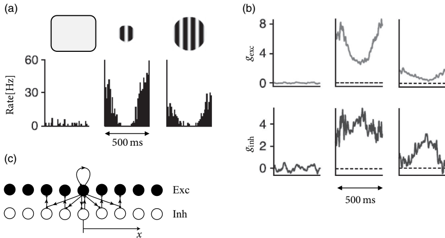
Fig. 18.13 Network stabilized by local inhibition. The schematic model could potentially explain why larger gratings lead not only to less excitatory input g_{exc} , but also to less inhibitory input g_{inh} . (a) The firing rate as a function of the phase of the moving grating for the three stimulus conditions (blank screen, small grating, and large grating). (b) Top: Excitatory input into the cell. Bottom: Inhibitory input into the same cell. As in (a), left, middle, and right correspond to a blank screen, a small grating, and a large grating. Note that the larger grating leads to a reduction of both excitation and inhibition. Adapted from Ozeki et al. (2009). (c) Network model with long-range excitation and local inhibition. Excitatory neurons within a local population excite themselves (feedback arrow), and also send excitatory input to inhibitory cells (downward arrows). Inhibitory neurons project to local excitatory neurons.
