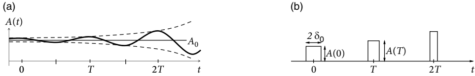
Fig. 20.5 Population activity A(t) during oscillations and synchrony. (a) An instability of asynchronous firing at rate A_0 leads to a sinusoidal oscillation of increasing amplitude. (b) If the fully synchronized state is stable, the width \delta_0 of the rectangular population pulses decreases while their amplitude A(kT) increases with each period.
