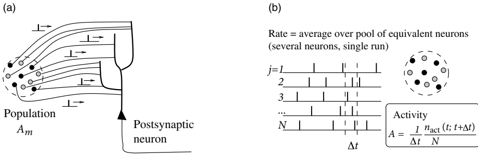
Fig. 7.8 (a) A postsynaptic neuron receives spike input from the population m with activity A_m . (b) The population activity is defined as the fraction of neurons that are active in a short interval [t, t + \Delta t] divided by \Delta t .
