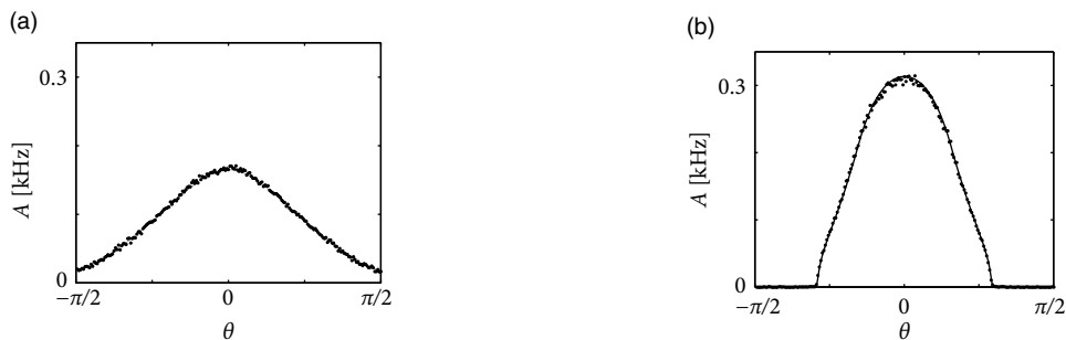
Fig. 18.11 Activity profiles in a model of orientation selectivity obtained by simulations based on \text{SRM}_0 neurons (dots) compared to the theoretical prediction (solid line) during stimulation with a low-contrast orientation input at \theta = 0 . (a) If lateral coupling is not distance-dependent [ \omega_2 = 0 ; see Eq. (18.20)] the activity profile reflects the weak modulation of the input pattern. (b) Excitatory coupling between cells of the same orientation and long-range inhibition ( \omega_2 = 10 ) generates a sharp activity profile centered at \theta = 0 . From Spiridon and Gerstner (2001) with permission of Informa Healthcare.
