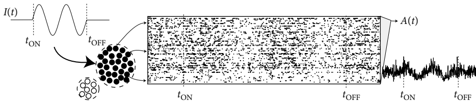
Fig. 12.2 Input and output of a population. A signal I(t) , represented by a sinusoidal modulation of the input starting at t_{ON} and ending at t_{OFF} , stimulates the population of 8000 excitatory neurons in a randomly coupled network of 8000 excitatory and 2000 inhibitory neurons (left). Each neuron produces a spike train (middle) illustrated here by lines of dots, each dot corresponding to a spike. Only 1% of the population is shown. The population activity A(t) (right) counts spikes in time bins of 1 ms averaged over the 8000 excitatory neurons.
