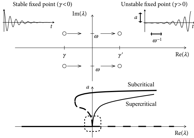
Fig. 4.16 Hopf bifurcation. Top: Complex plane of eigenvalues. When the bifurcation parameter increases, the real part of the complex eigenvalues \lambda_{+/-} = \gamma \pm i\omega passes at the bifurcation point from a negative value ( \gamma < 0 ) to a positive one. Associated stable and unstable oscillatory solutions are shown in left and right insets, respectively. Bottom: Amplitude a of oscillatory solutions as a function of \gamma . For \gamma < 0 the fixed point (constant solution) is stable corresponding to an oscillation of zero amplitude. At the bifurcation point, the constant solution loses its stability (dashed line) and a novel oscillatory solution appears. The amplitude of the oscillatory solution increases continuously. For a supercritical Hopf bifurcation the oscillatory solution is stable (solid line) whereas for a subcritical Hopf bifurcation, it is unstable close to the bifurcation point. The linear bifurcation analysis is valid only in the direct neighborhood of the bifurcation point (dashed box) and cannot predict the stable limit cycle (solid line) of the subcritical Hopf bifurcation.
