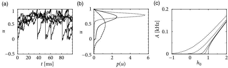
Fig. 13.5 (a) Membrane potential trajectories of five neurons ( R = 1 and \tau_m = 10 ms) driven by a constant background current I_0 = 0.8 and stochastic background input with \nu_+ = \nu_- = 0.8 kHz and w_{\pm} = \pm 0.05 . These parameters correspond to h_0 = 0.8 and \sigma = 0.2 in the diffusive noise model. (b) Stationary membrane potential distribution in the diffusion limit for \sigma = 0.2 (solid line), \sigma = 0.1 (short-dashed line), and \sigma = 0.5 (long-dashed line). (Threshold \vartheta = 1 .) (c) Mean activity of a population of integrate-and-fire neurons with diffusive noise as a function of h_0 for four different noise levels: (from top to bottom) \sigma = 1.0 , \sigma = 0.5 , \sigma = 0.2 (solid line), \sigma = 0.1 , \sigma = 0.0 .
