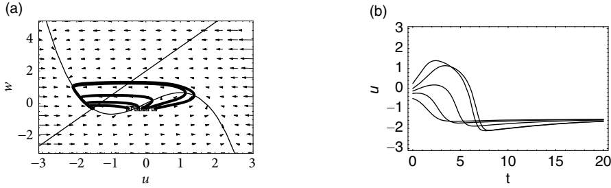
Fig. 4.20 Threshold behavior in a model with Hopf bifurcation. (a) Trajectories in the phase starting with initial conditions (u_0, w_{\text{rest}}) where u_0 = -0.5, -0.25, -0.125, 0, 0.25 . (b) Projection of the trajectories on the voltage axis. For u_0 \leq -0.25 , the trajectories return rapidly to rest. The trajectories with u_0 \geq -0.125 start with positive slope. Parameters were b_0 = 2, b_1 = 1.5, \varepsilon = 0.1 with I = 0 .
