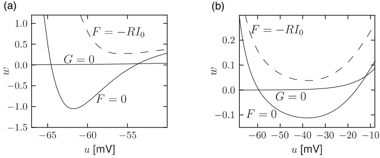
Fig. 4.4 Close-up of Fig. 4.3a and b. Solid lines: the sets of points with F(u, w) = 0 and G(u, w) = 0 are determined in the absence of stimulation ( I = 0 ). Dashed line: in the presence of a constant current I = I_0 > 0 , the set of points with du/dt = 0 is given F(u, w) = -RI_0 . The curve G(u, w) = 0 characterizing the points with dw/dt = 0 starts (for u \rightarrow -\infty ) nearly horizontally at w = 0 and does not change under stimulation.
