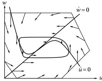
Fig. 4.9 Bounding surface around an unstable fixed point and the limit cycle (schematic figure).
