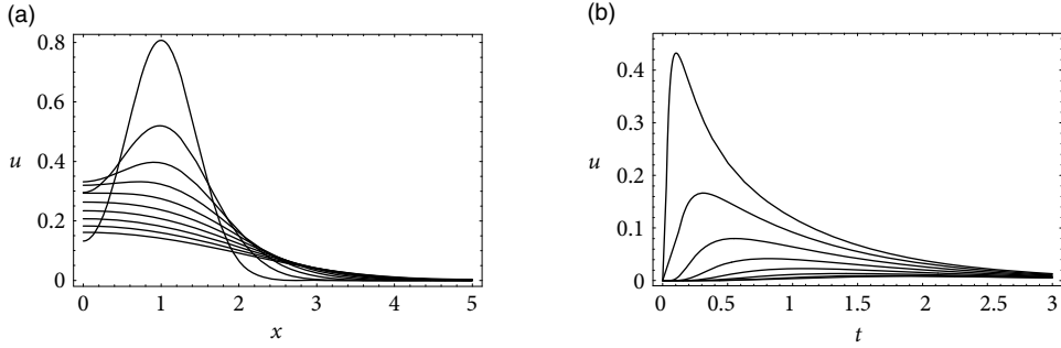
Fig. 3.7 Spatial distribution (a) and temporal evolution (b) of the membrane potential along a dendrite ( L = 5 ) with sealed ends ( \left. \frac{\partial u}{\partial x} \right|_{x \in \{0, L\}} = 0 ) after injection of a unit current pulse at x = 1 and t = 0 . The various traces in (a) show snapshots for time t = 0, 0.1, 0.2, \dots, 1.0 , respectively (top to bottom). The traces in (b) give the membrane potential as a function of time for different locations x = 1.5, 2.0, 2.5, \dots, 5.0 (top to bottom) along the cable.
