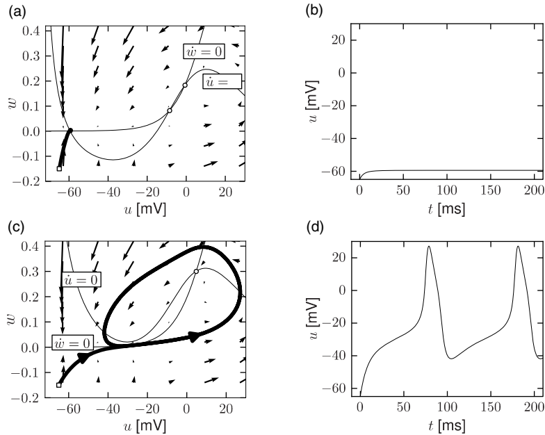
Fig. 4.13 (a) The nullclines of the Morris–Lecar model for zero input. The w -nullcline is flat at low u but increases monotonically above u = -20 , the u -nullcline is the nonlinear curve crossing the w -nullcline in three points. (a) Trajectory starting at (-65, -0.15) (open square) converges to the stable fixed point at (-59, 0) (filled circle). (b) Time course of the membrane potential of the trajectory shown in (a). (c) Same as in (a) but with positive input I = 45 . The stable fixed point in (a) has merged with the saddle (open circle in (a)) and disappeared leaving a limit cycle around the third, unstable, fixed point. (d) Voltage time course of the trajectory shown in (c). Trajectories are the results of numerical integration of Eqs. (4.6)–(4.10).
